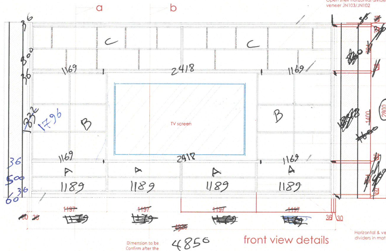
TV UNIT WITH SLIDING DOOR floor plan details
